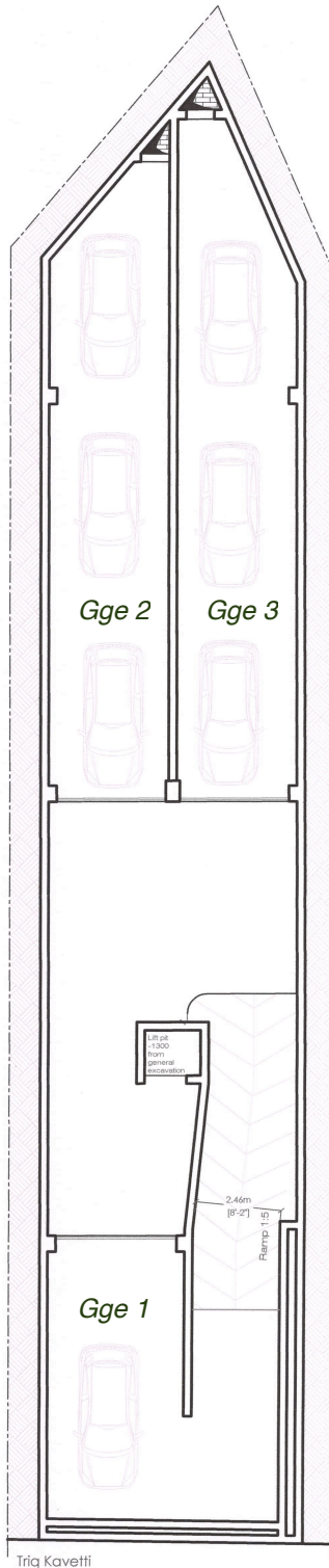
Basement Plan (level -1)
