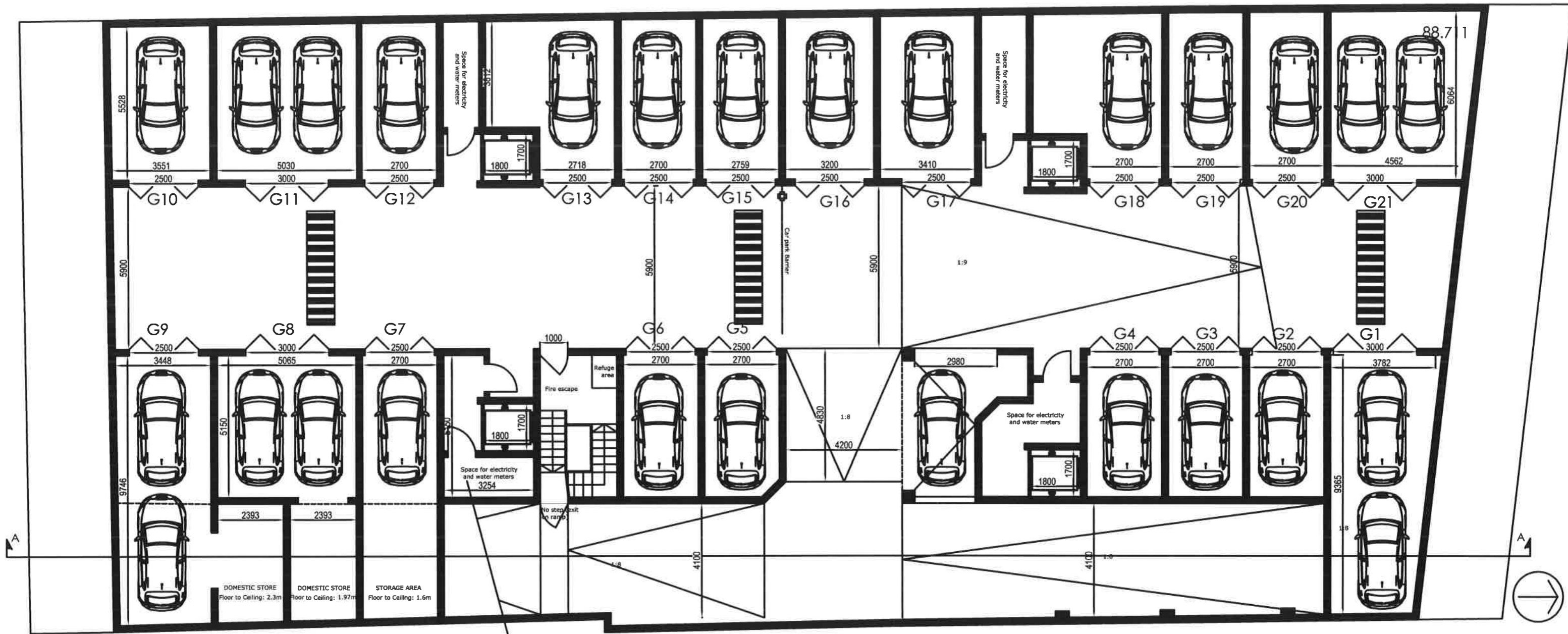
As-built Upper Basement Floor Level Scale 1:100
