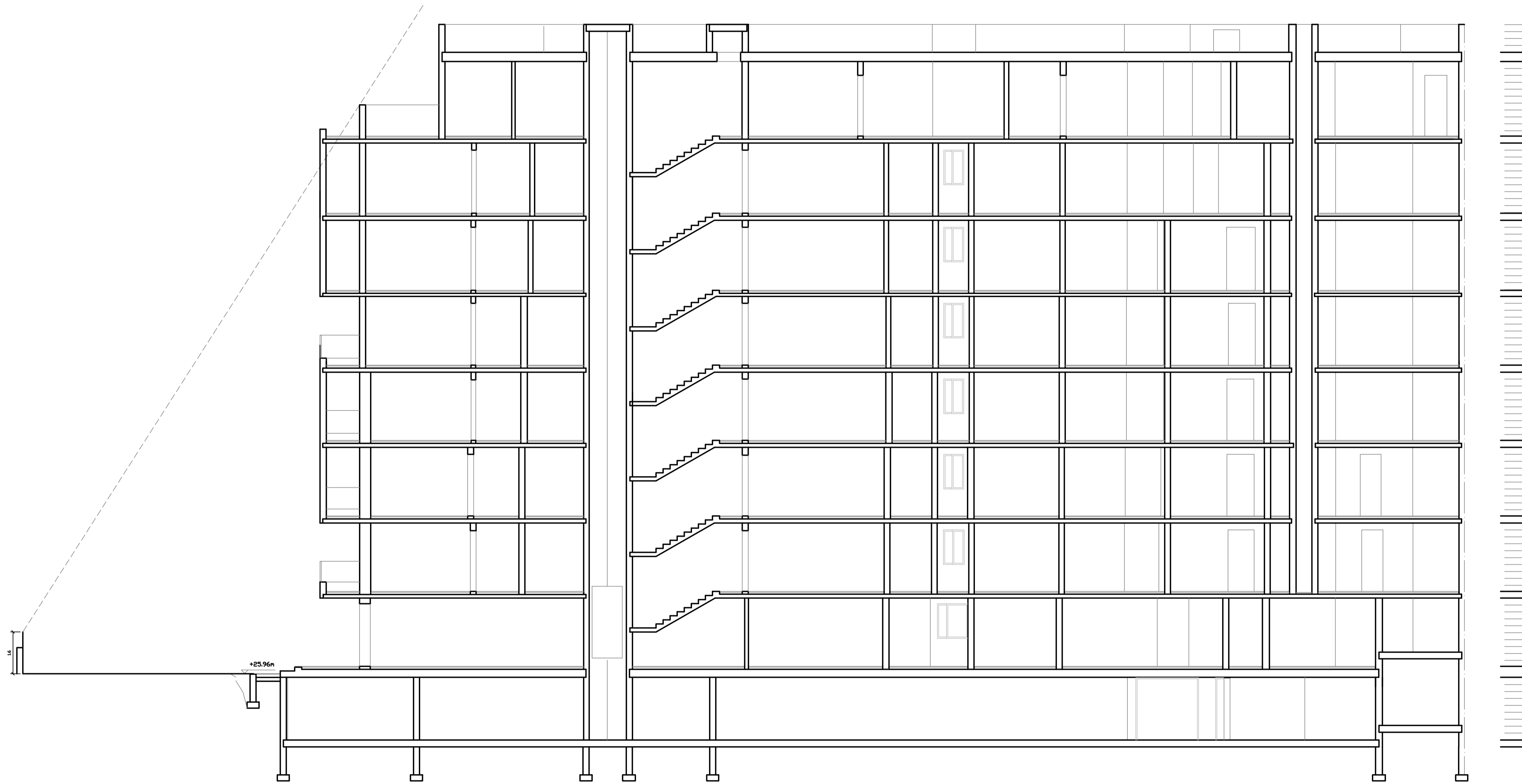
PROPOSED SECTION DW 11
