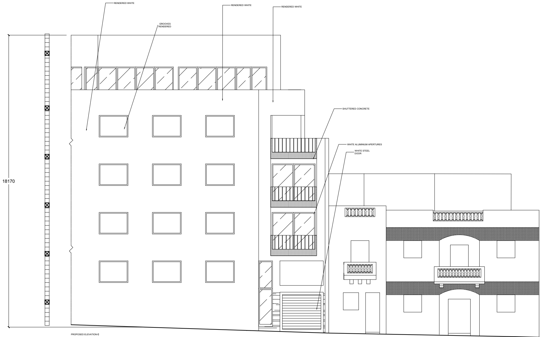
PROPOSED ELEVATION C
