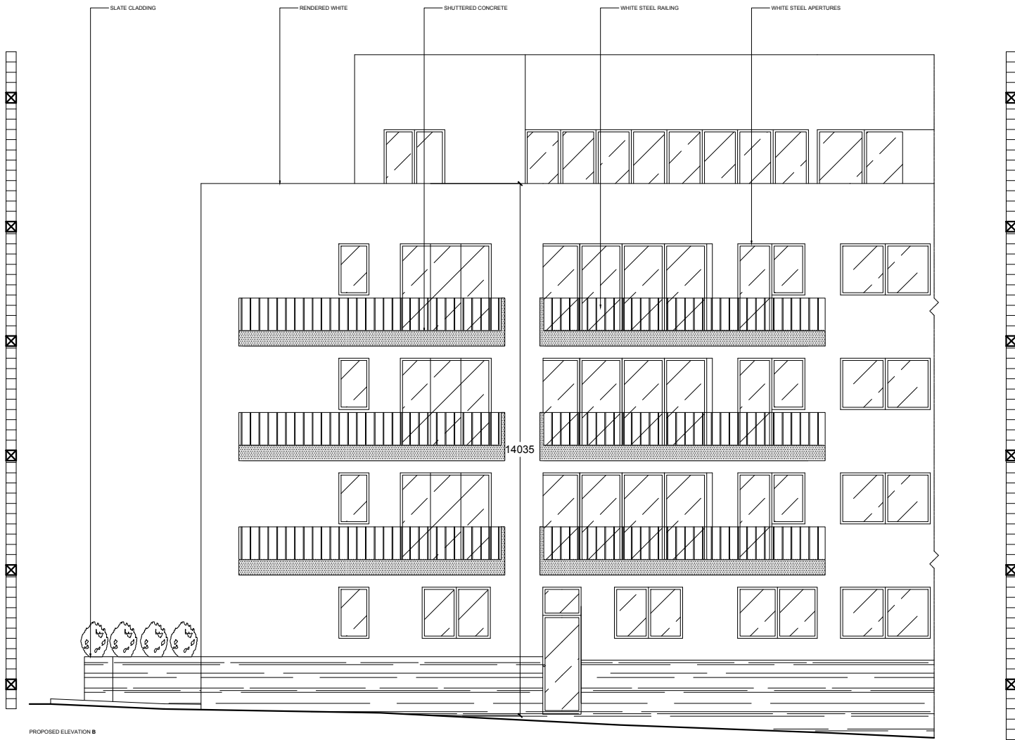
PROPOSED ELEVATION B
